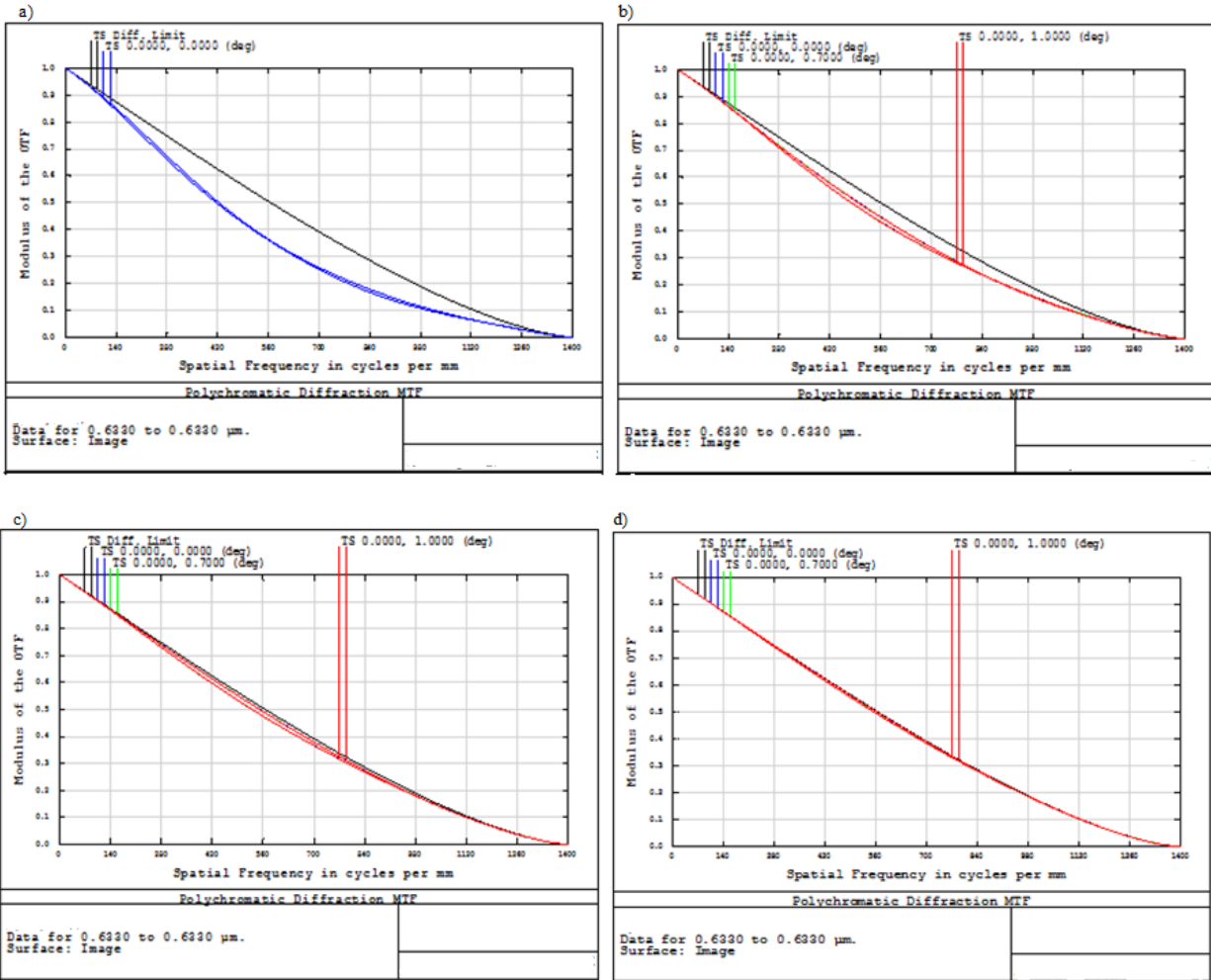
Figure 5: a) Uncompensated system performance of an F/1.0 paraxial lens with a 25cm aperture behind Window A. System MTF is reduced by 15% at 700 lp/mm. b) Uncompensated system performance of an F/1.0 paraxial lens with a 20cm aperture behind Window A. System MTF is slightly impacted by approximately 5% at 700 lp/mm. c) Uncompensated system performance of an F/1.0 paraxial lens with a 15cm aperture behind Window A. System MTF is essentially unaffected and shows nearly diffraction limited performance. d) Uncompensated system performance of an F/1.0 paraxial lens with a 10cm aperture behind Window A. System demonstrates diffraction limited performance.
