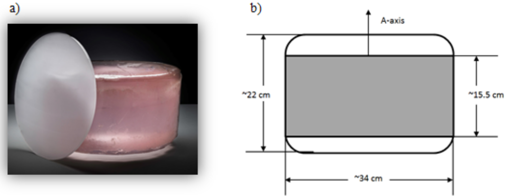
Figure 1: a) A typical boule produced from the HEM method with a representative blank; b) Typical dimensions of an as-grown HEM boule. The area shown in grey represents the portion of the boule which is considered optical quality.
