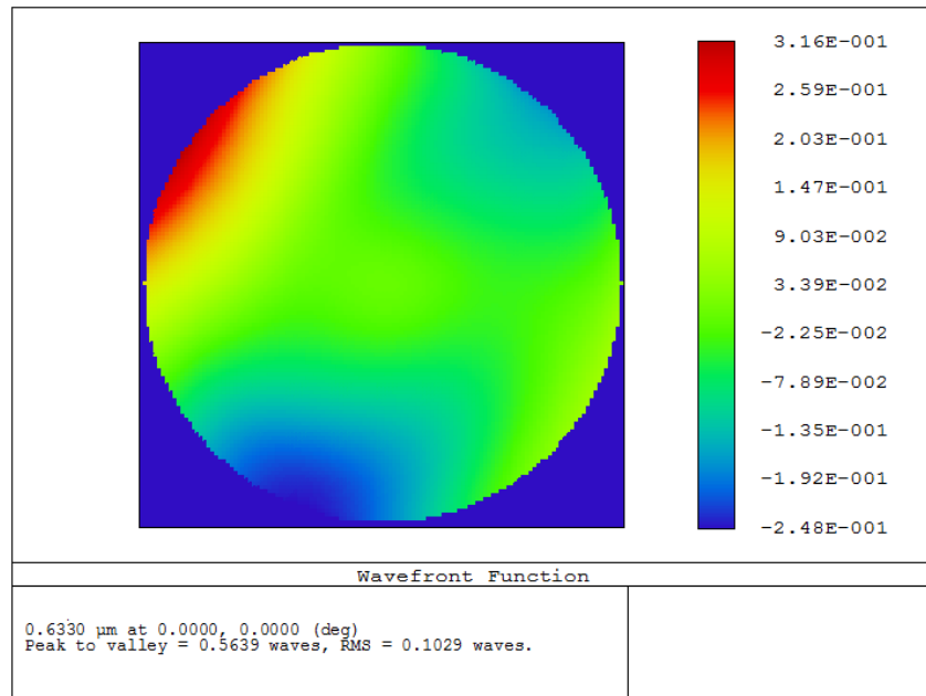
Figure 3: Simulated TWE for sapphire Window A. Primary aberration due to inhomogeneity is astigmatism.
