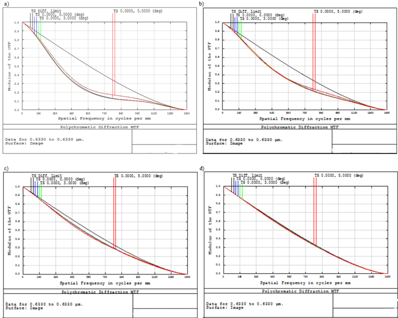
Figure 6: a) Uncompensated system performance of an F/1.0 paraxial lens with a 25cm aperture behind Window B. System MTF takes a significant hit by 30% at 570 lp/mm before focus compensation due to power caused by the inhomogeneity of Window B. b) Uncompensated system performance of an F/1.0 paraxial lens with a 20cm aperture behind Window B. System MTF is impacted by 15% at 570 lp/mm. c) Uncompensated system performance of an F/1.0 paraxial lens with a 15cm aperture behind Window B. System MTF is slightly reduced by <5% due to the power caused by the inhomogeneity of Window B. d) Uncompensated system performance of an F/1.0 paraxial lens with a 10cm aperture. System demonstrates near diffraction limited performance.
