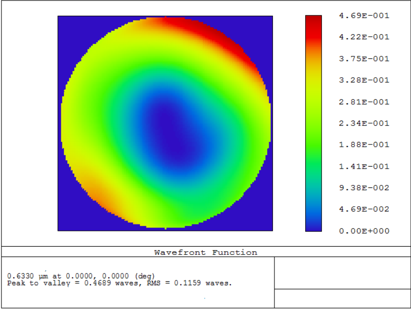
Figure 4: Simulated TWE for sapphire Window B. Primary aberration due to inhomogeneity is power.
