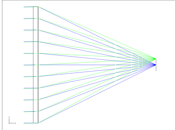
Figure 2: Model used for evaluation of MTF impact due to TWE of index inhomogeneity in a sapphire window. Model depicts sapphire window with a Zernike fringe on the rear surface and an ideal paraxial lens directly behind the window for image evaluation.
