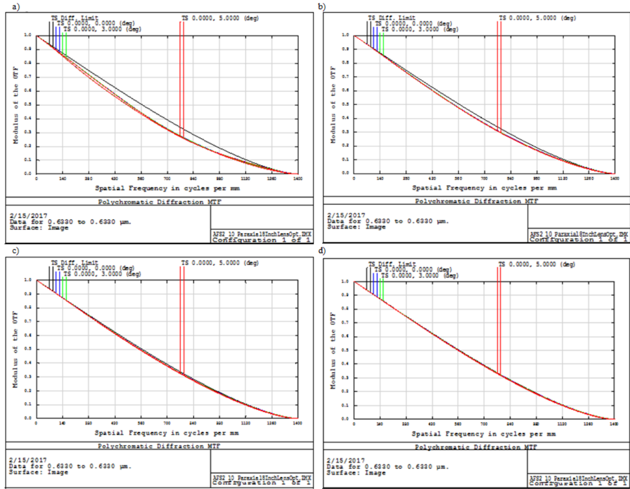
Figure 7: Compensated system performance of an F/1.0 paraxial lens behind Window B. System MTF losses can be focus compensated. a) 25cm aperture, b) 20cm aperture, c) 15cm aperture and d) 10cm aperture.
